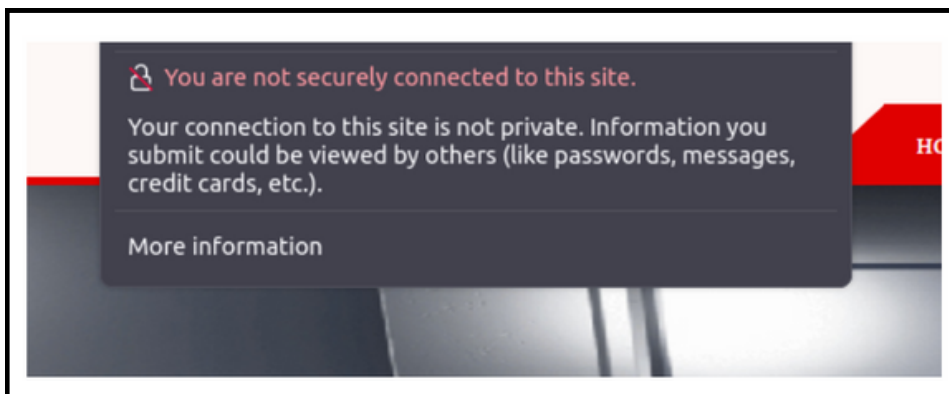
Fig 3: No HSTS
